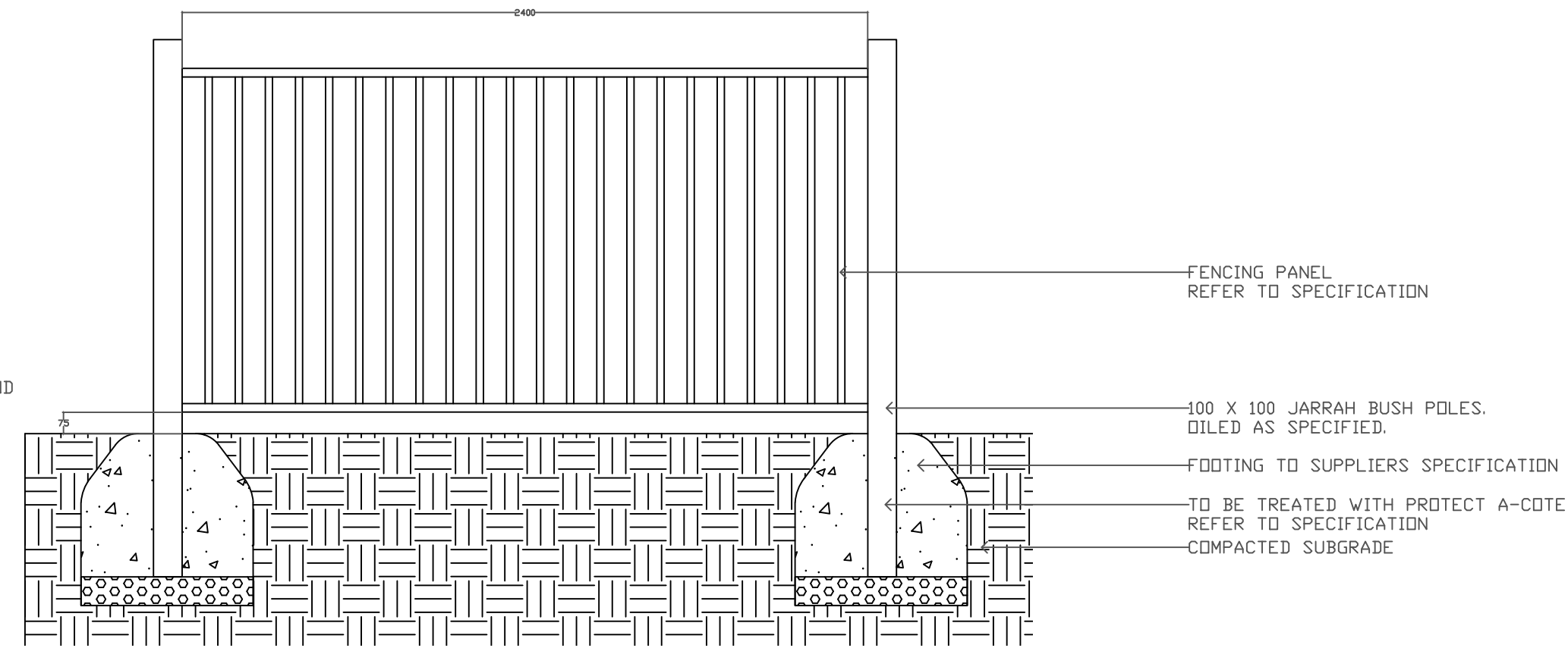
07 FENCE D01 SECTION SCALE 1:20
