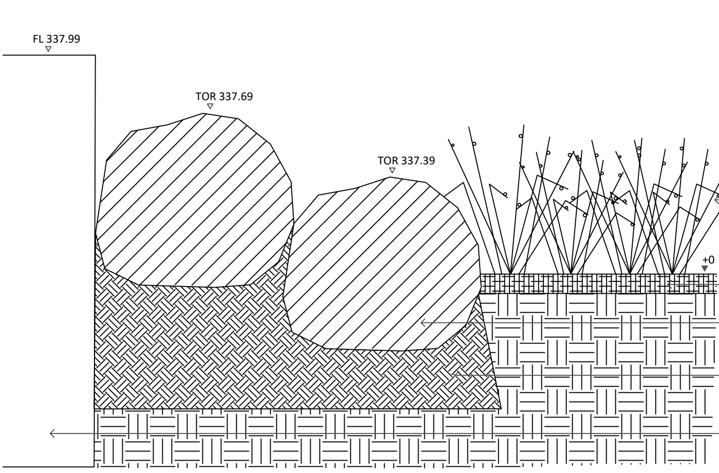
01 BOULDER EDGE TO SKATEPARK D01 SECTION SCALE 1:20
